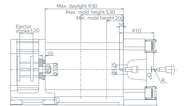
Clamping unit
