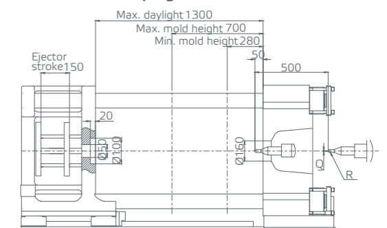
Clamping unit
