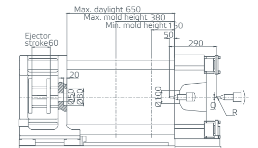
Clamping unit
