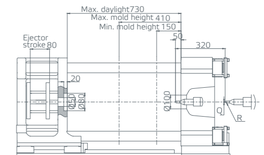
Clamping unit
